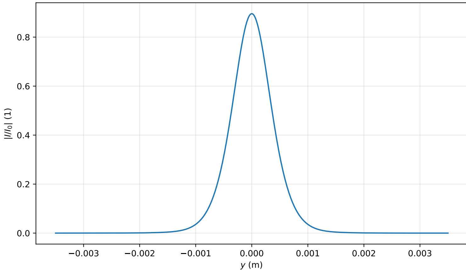
Intensity profile I(x=0, y, z=2.786)/I_0 , P_{in}=0.7P_{cr} , artificial time
